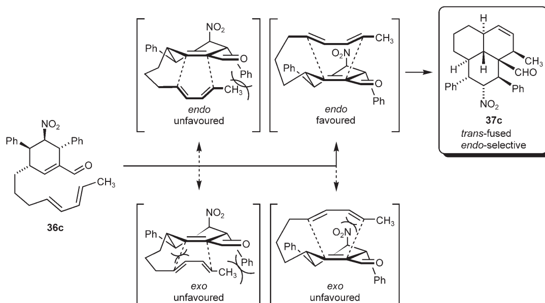
Figure 11. Proposed transition state leading to decahydrophenalene 37c ( n=1 ).
