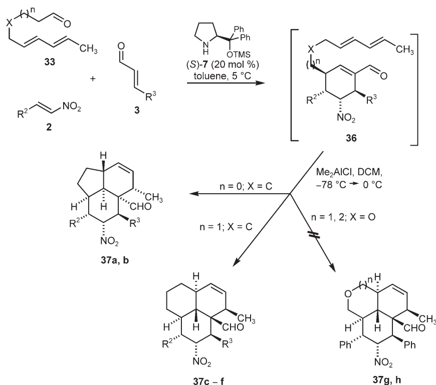
Scheme 9. One-pot synthesis of the decahydroacenaphthylene and decahydrophenalene derivatives 37 .
