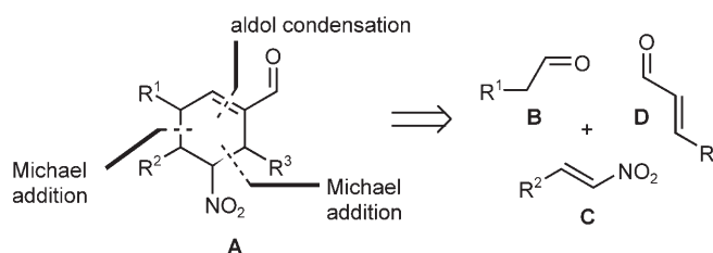
Figure 1. Retrosynthetic analysis of the triple cascade for the synthesis of the cyclohexene-carbaldehydes A .
