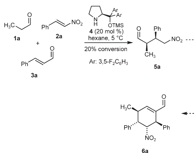
Scheme 1. First test reaction for the development of the three-step domino reaction of 6a .
