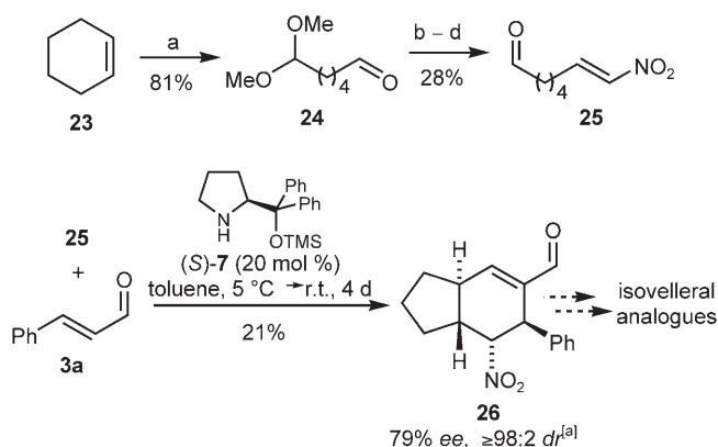
Scheme 6. Triple cascade for the synthesis of hexahydro-1 H -indene-carbaldehyde 26 ( [a] after chromatography): a) \text{O}_3 , DCM/MeOH (5:1), -78^\circ\text{C} ; p -TSA, r.t.; then \text{NaHCO}_3 ; DMS, r.t.; b) \text{MeNO}_2 , i -PrOH, KF, 0^\circ\text{C} \rightarrow \text{r.t.} ; c) DCC, cat. \text{Cu(I)Cl} , \text{Et}_2\text{O} , 0^\circ\text{C} \rightarrow \text{r.t.} ; d) p -TSA, acetone/ \text{H}_2\text{O} (4:1), \Delta , 1.5 h.
