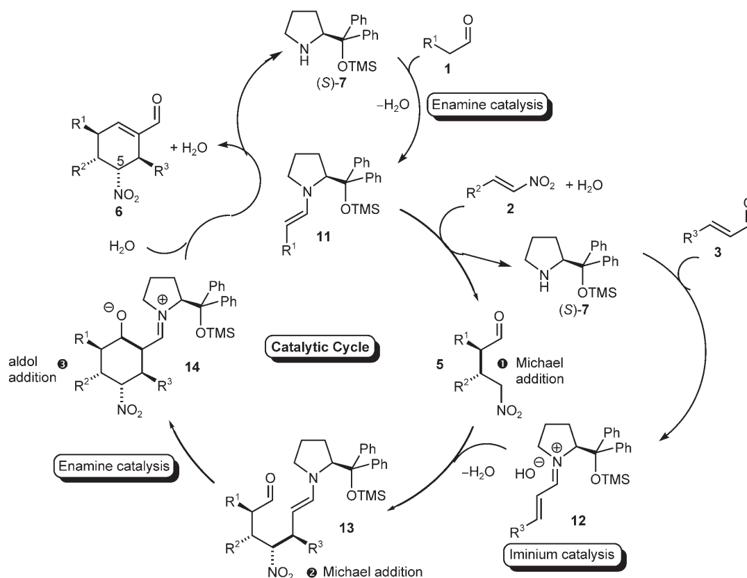
Figure 2. Proposed catalytic cycle of the triple cascade.
