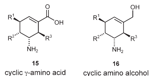
Figure 5. Synthetically interesting derivatives 15 and 16 .
