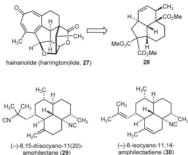
Figure 7. Structures of hainanolide ( 27 ), which can be traced back to 28 and amphilectanes 29 and 30 .
