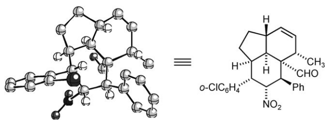
Figure 9. X-Ray structure analysis of decahydroacenaphthylene 37b . [22,30]
