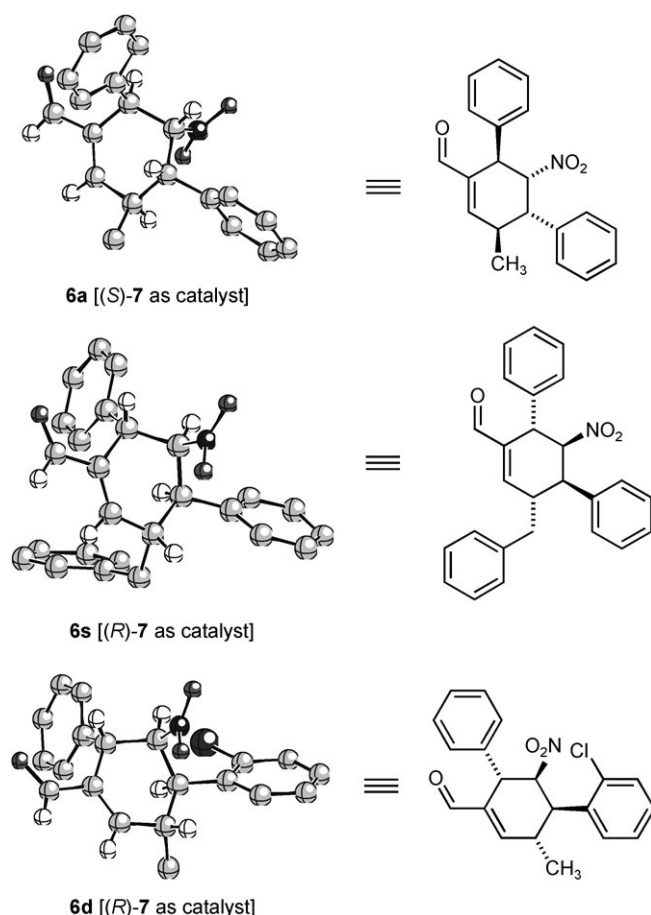
Figure 3. X-Ray structures of the cyclohexene-carbaldehydes 6a , 6s and 6d .
