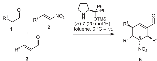
Scheme 2. Variation of the substrates 1 , 2 and 3 of the triple cascade.
