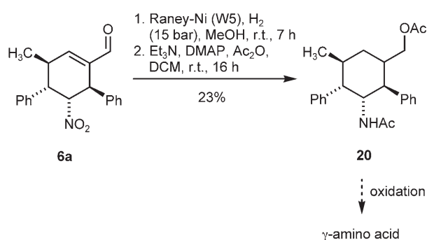
Scheme 5. Raney-Ni reduction of 6a and subsequent protection of the resulting amino alcohol to 20 .
