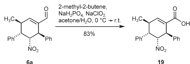
Scheme 4. Oxidation of 6a to the corresponding carboxylic acid 19 .
