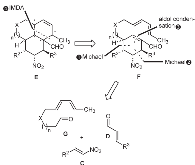
Figure 8. Retrosynthetic analysis of the tricyclic carbaldehyde E in four steps.
