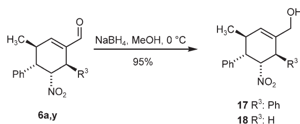
Scheme 3. \text{NaBH}_4 reduction of 6a and y to the corresponding alcohols 17 and 18 .
