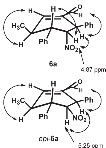
Figure 4. Representative enhancements of 6a and epi-6a .
