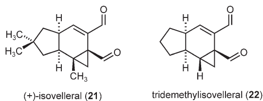
Figure 6. Structures of (+)-isovelleral ( 21 ) and tridemethylisovelleral ( 22 ).
