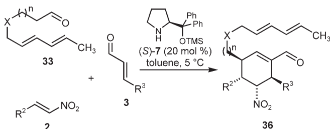
Scheme 8. Synthesis of the cyclohexene-carbaldehydes 36 bearing the diene moiety.
