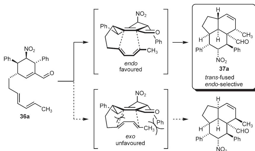
Figure 10. Proposed transition state leading to decahydroacenaphthylene 37a ( n=0 ).
