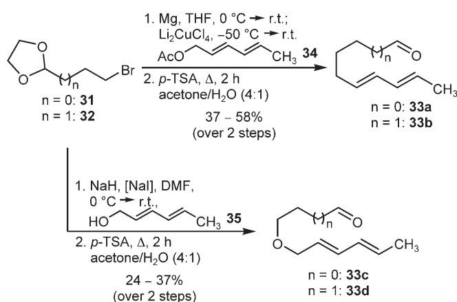
Scheme 7. Synthesis of the diene aldehydes 33a–d .
